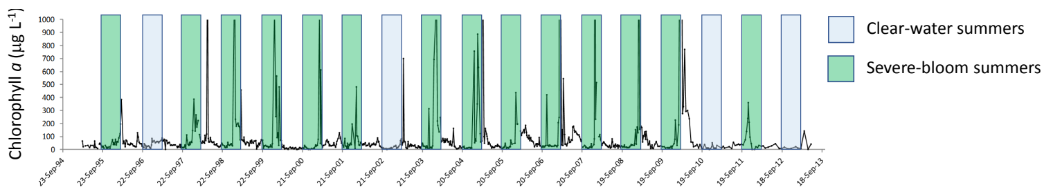
Figure 3. Time series of Wairewa/Lake Forsyth algal biomass time series data from 1994 to 2013, illustrating the instability (lack of resilience) of this lake. The instability can be observed in inter-annual differences in summer chlorophyll a maxima.
