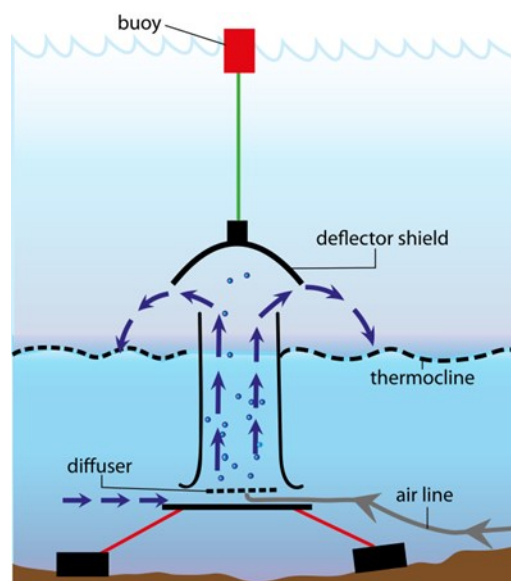
Figure 2. Conceptual diagram of destratification device in operation
