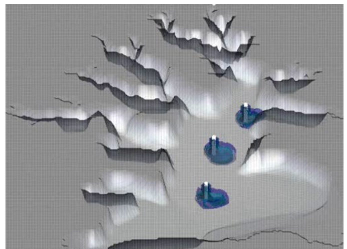
Figure 5. Model output showing three destratification devices in Lake Rotoehu. Image: Kohji Muraoka
